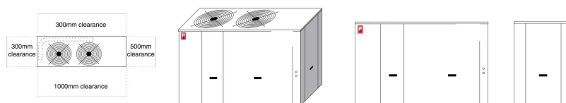
Installation clearances and unit views, dimensions in millimetres
