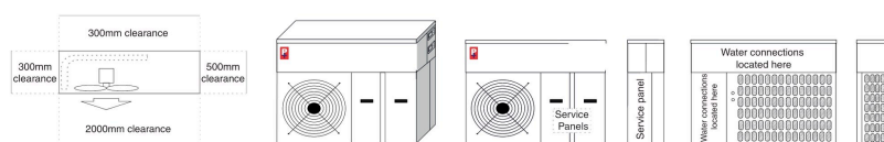
Installation clearances and unit views, dimensions in millimetres
