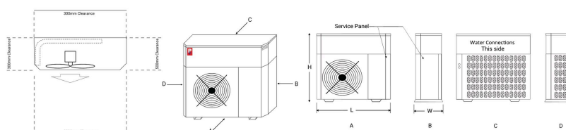
Installation clearances and unit views, dimensions in millimetres
