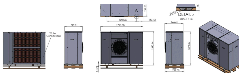
Installation clearances and unit views, dimensions in millimetres
