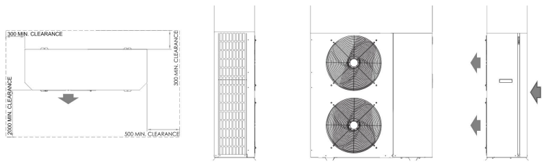
Installation clearances and unit views, dimensions in millimetres
