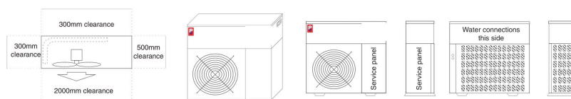
Installation clearances and unit views, dimensions in millimetres
